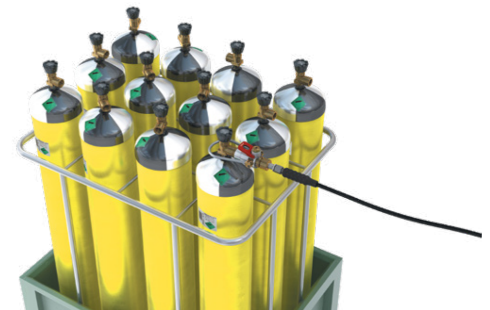
Hose filling system with CLICKMATE® TW154
