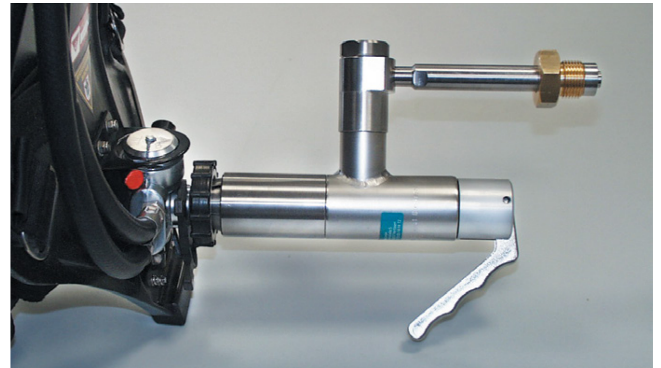
Testing of respiratory equipment with TW156 quick connector
