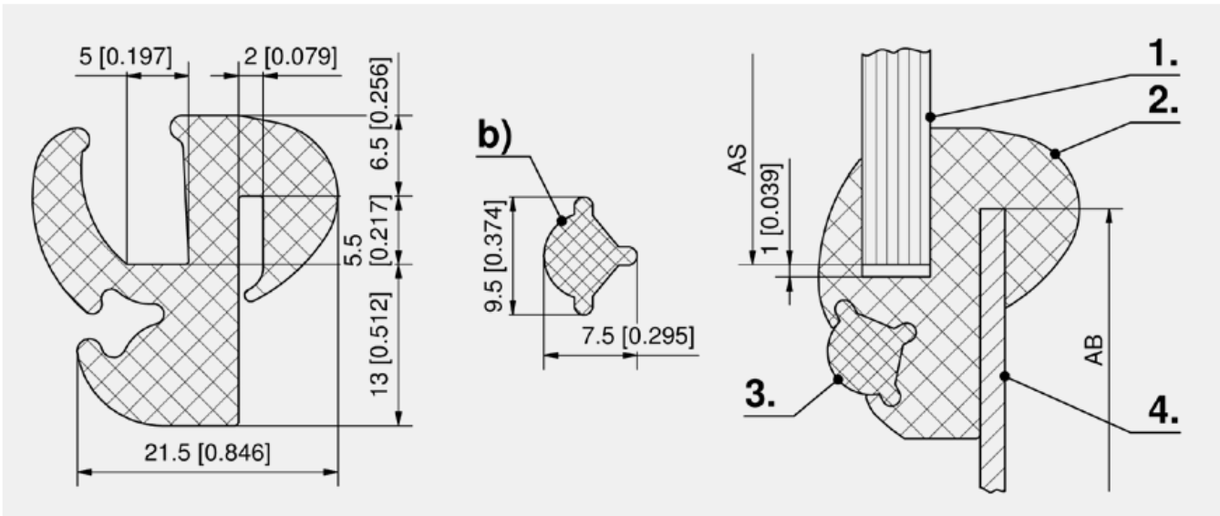
Window Seal
