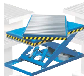
version with roller conveyor and slewing ring
