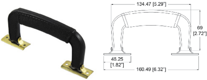
Black Plastic Attaché Handle
