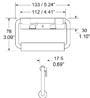
Extrusion Mount Field Dressed Spring-Loaded Handle.
