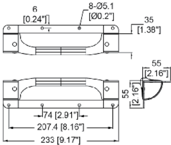
CUTOUT: 170 x 35 [6.69" x 1.34"]
