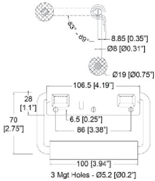
2356 Surface Mount Spring-Loaded Handle.
