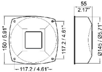
4 Fixing Holes Ø5.2 / Ø0.2"
