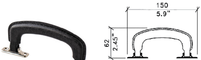
FIXING HOLES 4mm / .16" DIA
