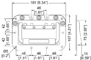
CUTOUT: 75 x 128 [2.95" x 5.04"] Material: 1.2mm / 18 gauge Steel
