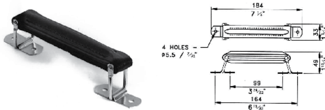
Leather Handle. Suits Backplates H1000/BP (p.98)
