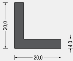
Part-Nr. 5400.2020 EPDM · 65° ShoreA · schwarz · VE: Bund á 50m
