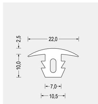
Part-Nr. 5540.3612 Silikon · 60° ShoreA · weiss VE: Bund á 50m
