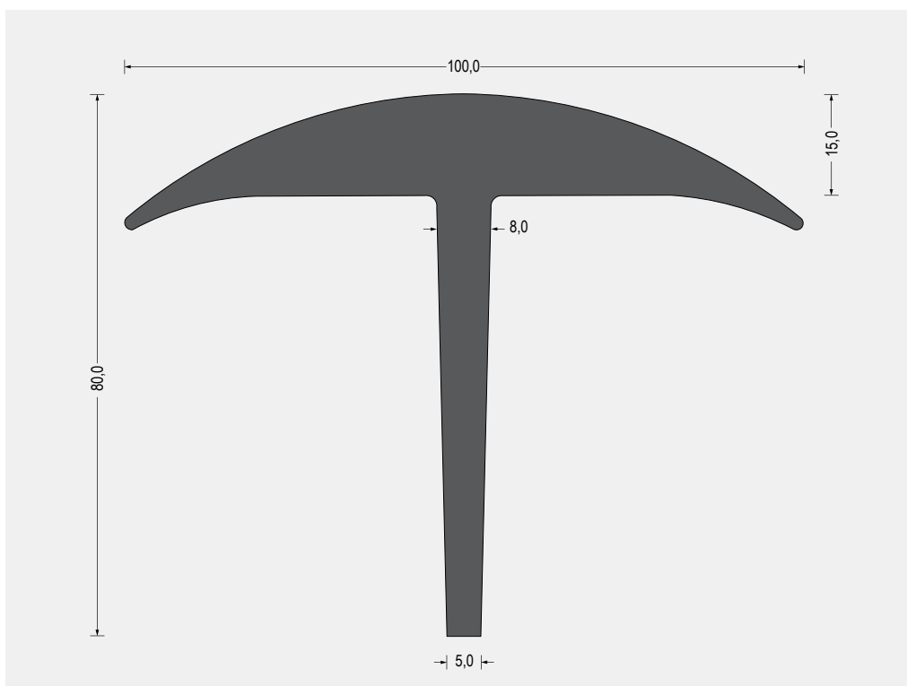
Part-Nr. 5500.3699 EPDM · 70° ShoreA · schwarz VF: Bund á 18.1m
