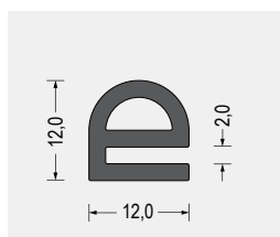
Part-Nr. 5500.2012 EPDM · 65° ShoreA · schwarz VE: Bund á 50m
