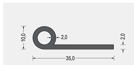
Part-Nr. 5400.5102 EPDM · 60° ShoreA · schwarz VE: Bund á 50m
