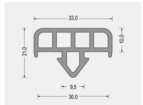
Part-Nr. 5470.4256 Weich-PVC · 70° ShoreA · grau VE: Bund á 50m
