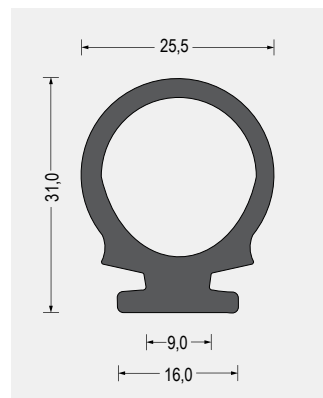
Part-Nr. 5470.3109 Weich-PVC · 65° Shore A · schwarz VE: Bund á 40m
