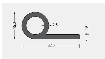
Part-Nr. 5400.5154 EPDM · 70° ShoreA · schwarz VE: Bund á 50m
