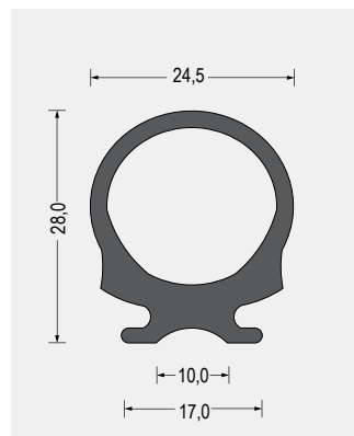
Part-Nr. 5470.3059 Weich-PVC · 65° Shore A · schwarz VE: Bund á 40m
