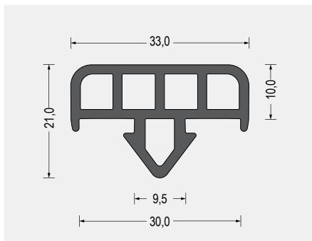
Part-Nr. 5470.4259 Weich-PVC · 70° ShoreA · schwarz VE: Bund á 50m
