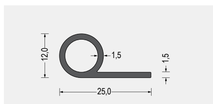
Part-Nr. 5400.5122 EPDM · 60° ShoreA · schwarz VE: Bund á 50m
