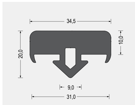
Part-Nr. 5400.4239 EPDM · 70° ShoreA · schwarz VE: Bund á 25m
