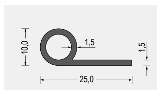
Part-Nr. 5420.5101 NBR · 60° ShoreA · schwarz VE: Bund á 50m
