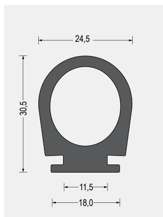
Part-Nr. 5400.3079 EPDM · 65° Shore A · schwarz VE: Bund á 50m
