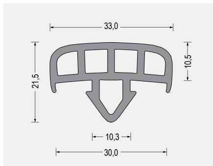
Part-Nr. 5470.4356 Weich-PVC · 85° ShoreA · grau VE: Bund á 30m
