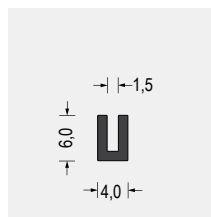
Part-Nr. 5500.0171 EPDM · 60° ShoreA schwarz VE: Bund á 200m
