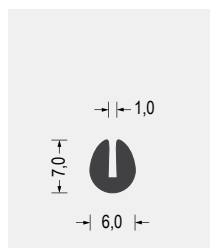
Part-Nr. 5530.0101 EPDM · 70° ShoreA schwarz VE: Bund á 100m
