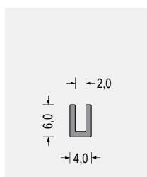
Part-Nr. 5540.0236 60° ShoreA · grau VE: Bund á 50m
