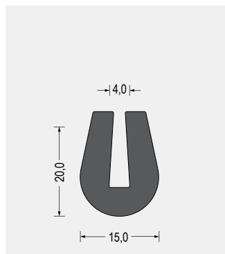
Part-Nr. 5500.0488 EPDM · 65° ShoreA · schwarz VE: Bund á 50m
