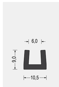
Part-Nr. 5500.0604 EPDM · 65° ShoreA schwarz VE: Bund á 50m
