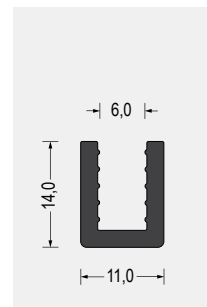
Part-Nr. 5570.0601 Weich-PVC · 74° ShoreA schwarz VE: Bund á 100m
