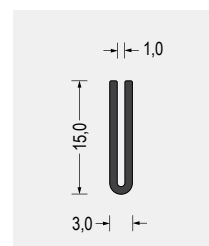
Part-Nr. 5500.0101 EPDM · 65° ShoreA schwarz VE: Bund á 100m
