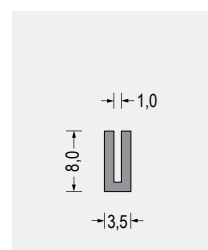
Part-Nr. 5540.0127 60° ShoreA · grau VE: Bund á 50m
