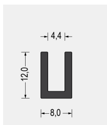
Part-Nr. 5500.0476 EPDM · 65° ShoreA schwarz VE: Bund á 100m
