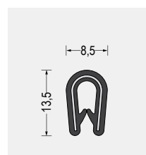
Part-Nr. 5610.0469 Soft Rubber EPDM schwarz Klemmbereich 1-2,5mm VE: Bund á 100m
