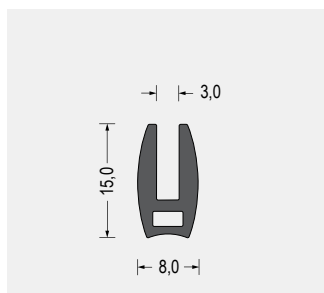
Part-Nr. 5500.0366 EPDM · 65° ShoreA · schwarz VE: Bund á 50m
