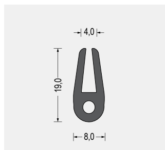
Part-Nr. 5500.0472 EPDM · 65° ShoreA · schwarz VE: Bund á 50m
