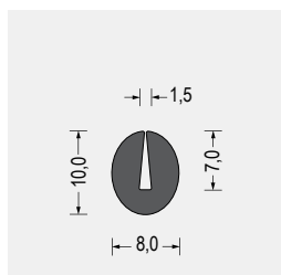
Part-Nr. 5800.9672 EPDM · schwarz VE: Bund á 100m
