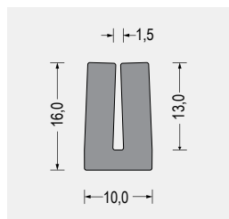
Part-Nr. 5800.7711 EPDM · grau VE: Bund á 50m
