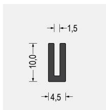
Part-Nr. 5500.0179 EPDM · 75° ShoreA schwarz VE: Bund á 50m
