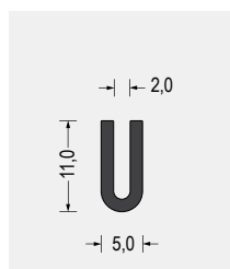
Part-Nr. 5570.0201 Weich-PVC · 57° ShoreA schwarz VE: Bund á 200m
