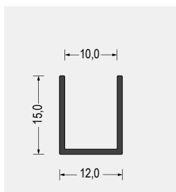
Part-Nr. 5500.1022 EPDM · 65° ShoreA schwarz VE: Bund á 50m
