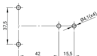
Mounting hole
