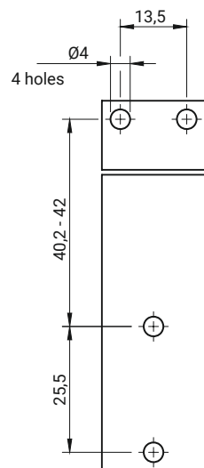
Mounting hole
