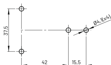
Mounting hole
