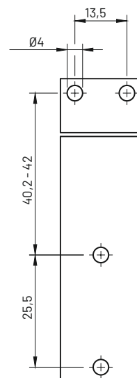
Mounting hole 3.562.002
