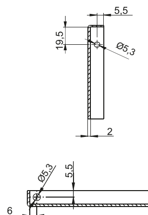
3.ST96.003 3.ST96.004
