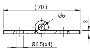
3.ST30.001
