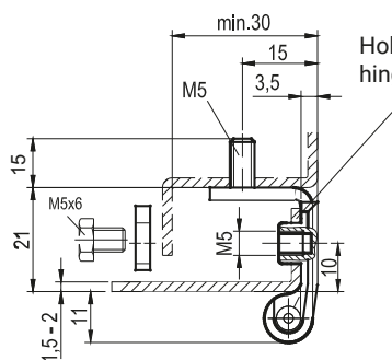
3.ZN120.002
