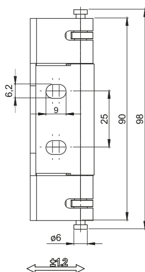
3.ST12B.002
