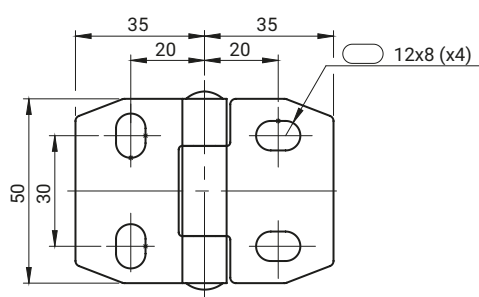
3.ST30.010
