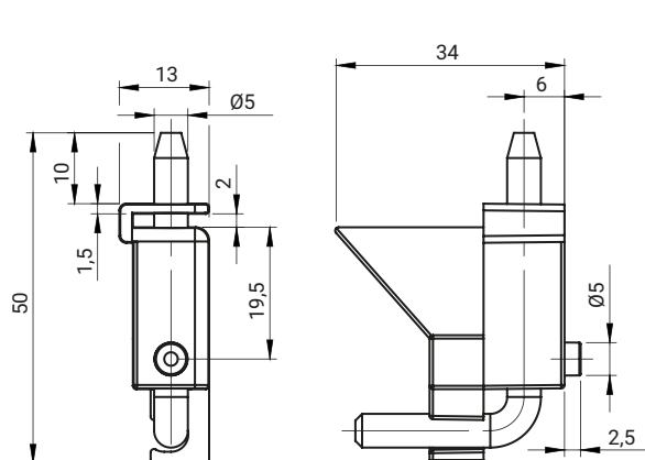
3.ST96.004
