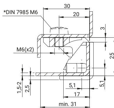
3.ZN80.003SN
