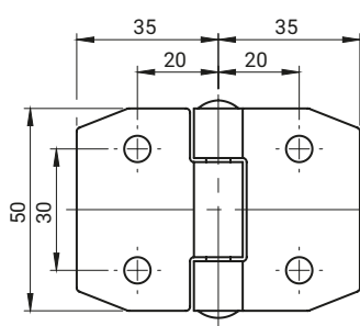
3.ST30.008
