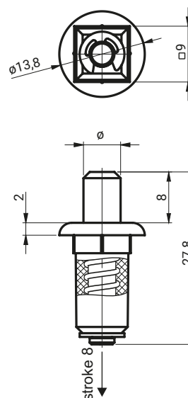
3.ST81.100 3.ST81.101
