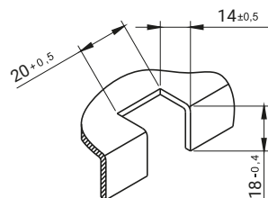
Mounting hole
