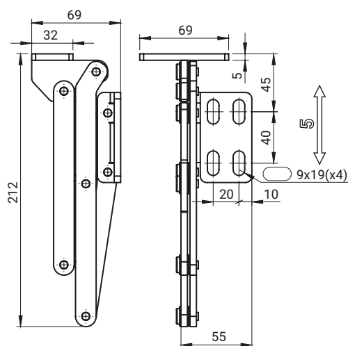
3.ST305.001
