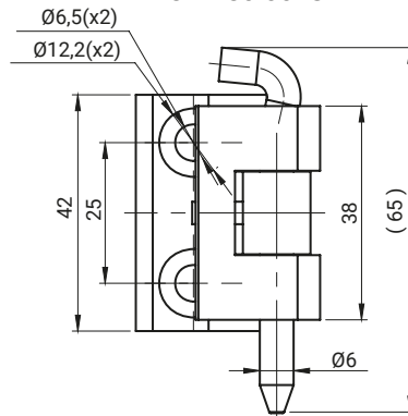
3.ZN80.004SN
