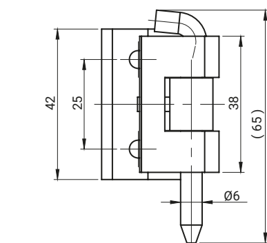
3.ZN80.003SN
