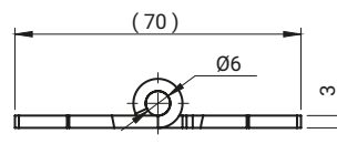
3.ST30.005
