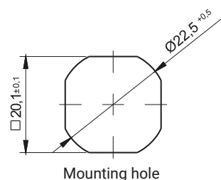
Mounting hole
