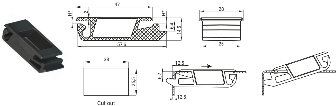
Cut out
