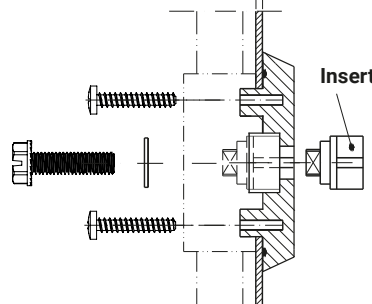
RW110.M ... (Used with Cogwheel mechanism)
