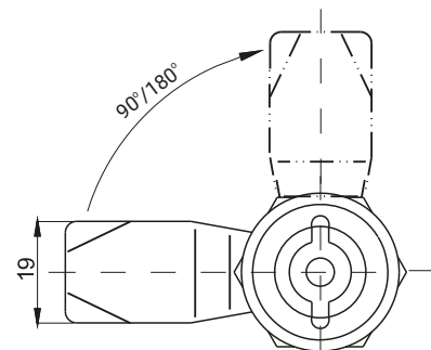
Right version
