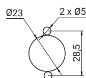
Cut out
