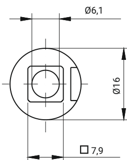
ADAPTER 1C.903.001
