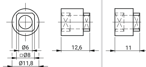
1C.901.001
